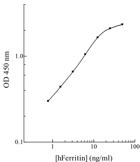
Human Ferritin Standard Curve
